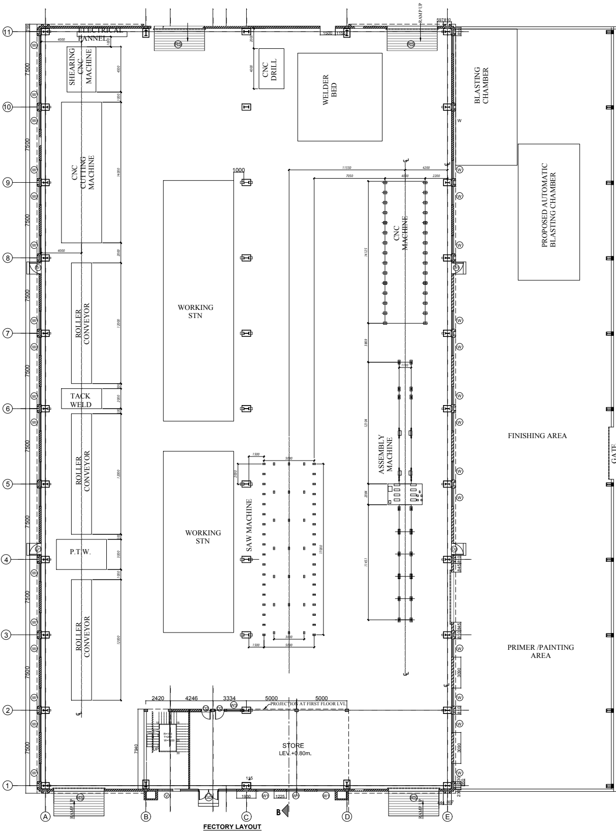
FACTORY LAYOUT
